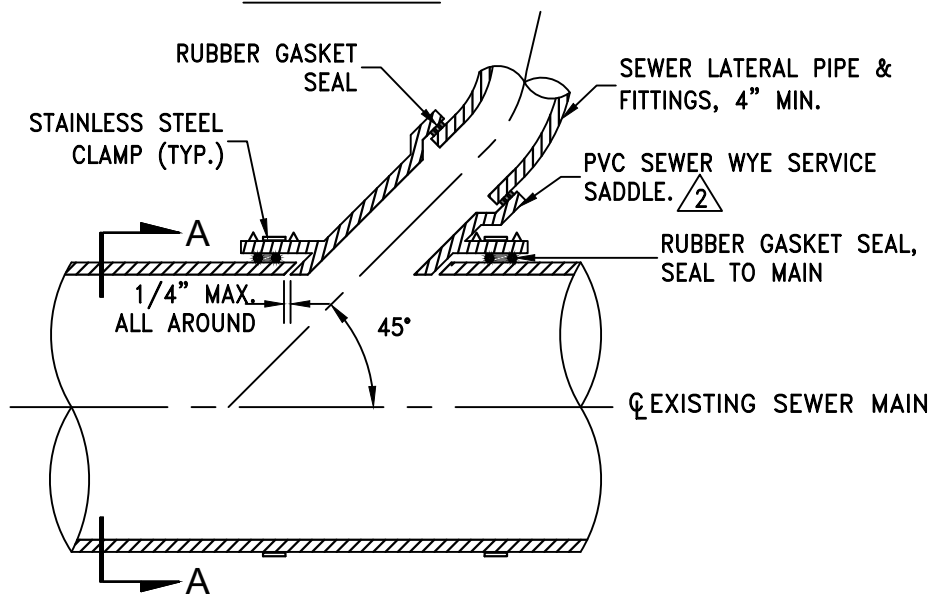
SIDE VIEW
