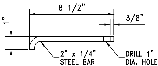
LOCKING BAR
