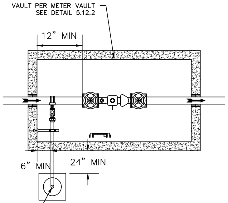
PLAN VIEW
