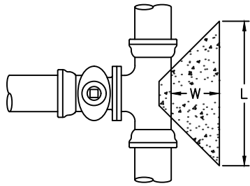
TEE / TAPPING SLEEVE PLAN VIEW
