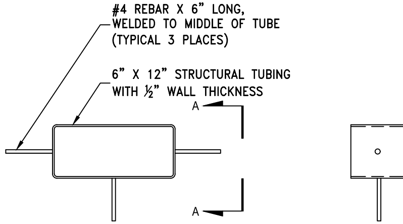
TUBING DETAIL
