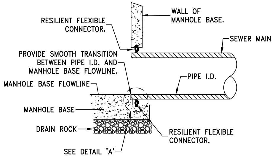
SECTION
